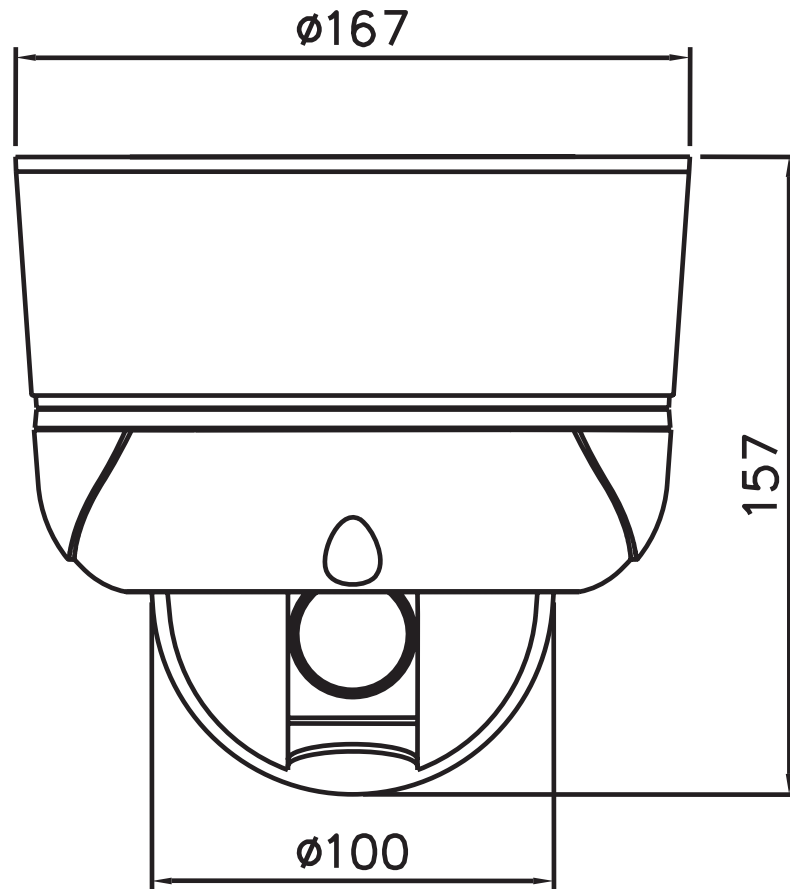
TH-Z1021/TH-Z1021 H
