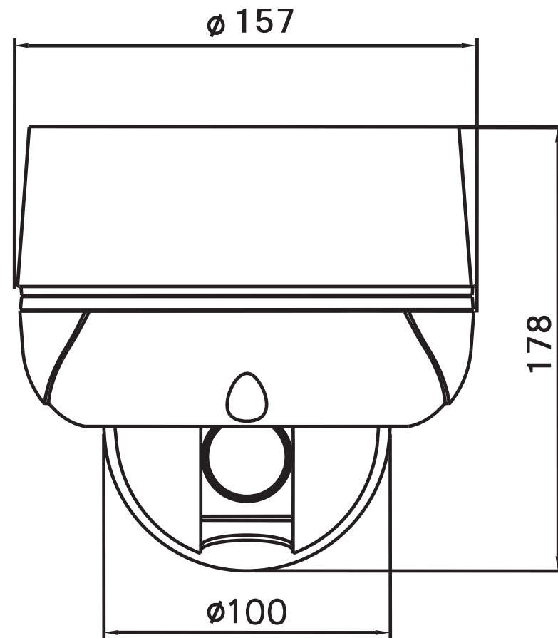
TH-Z1021 IP
